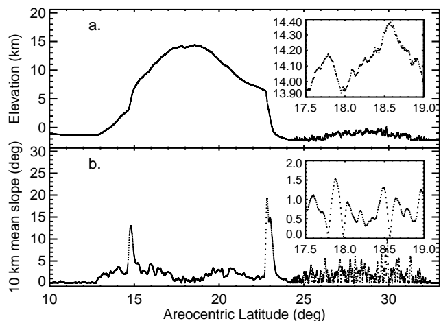
Figure 2. Topography (a) and slopes (b) across the Olympus Mons shield (Pass 24; longitude -138^\circ E). A portion of the profile running west of the volcano's summit is shown in the insert.
